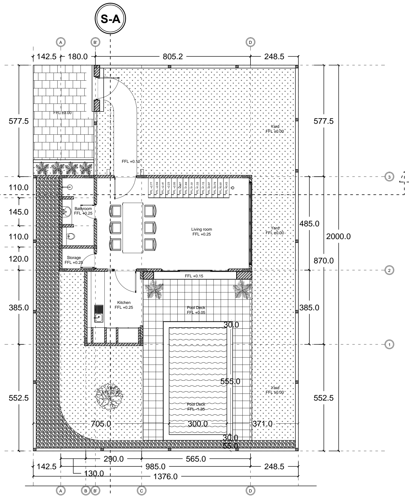
Ground Floor Mezzanine Villa Scale 1:100
